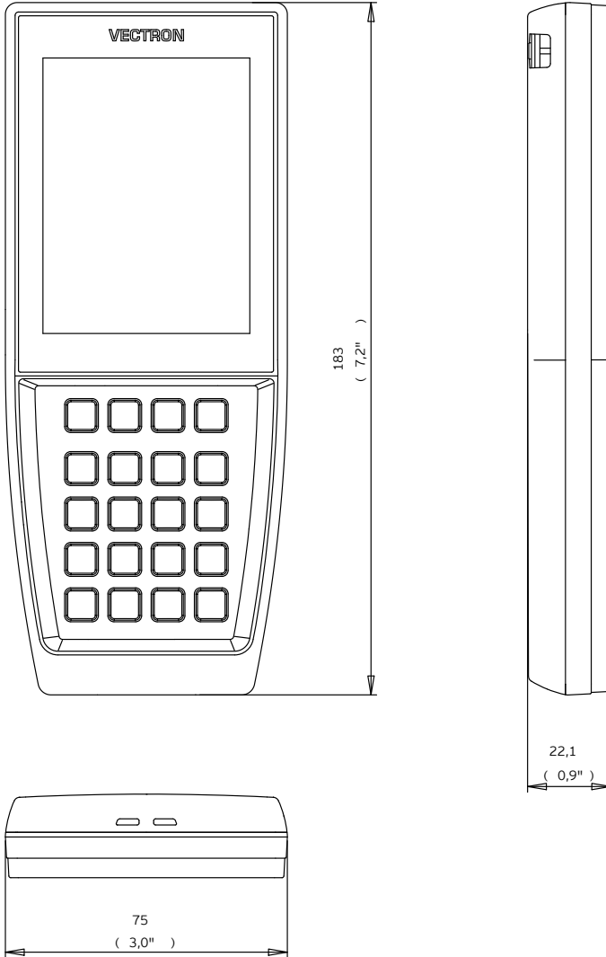
Fig. 13: POS MobilePro III (in mm and inch)
